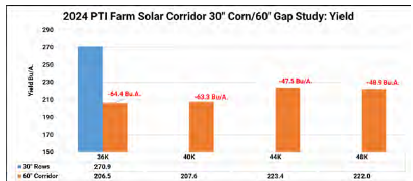
Figure 1. 60" Solar Corridor Corn System
